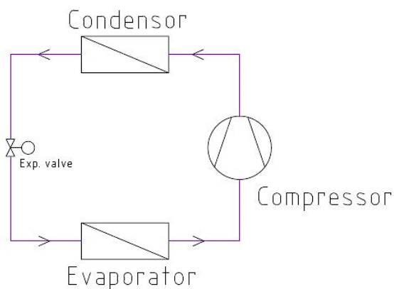
Fig 2. Principal layout showing the refrigerant circuit.
